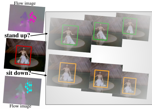
Figure 1: Two-in-one stream. We propose to embed RGB and optical-flow into a single stream for spatio-temporal action detection. Besides efficiency gains, it helps recognizing whether the dancer in the current frame is standing up or sitting down without considering the future. By utilizing information from flow images, the dancer is given a moving direction, up or down, better indicating the action.
