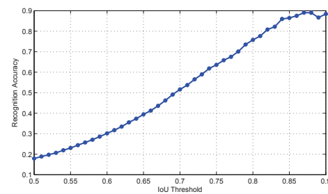
Fig. 10: The relation between the ground-truth overlap threshold (i.e., the IoU threshold) and the word recognition accuracy, evaluated on SVT dataset [55]. Proposals with higher IoU values are better recognizable.
