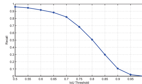
Fig. 11: The influence of the ground-truth overlap threshold (i.e., the IoU threshold) on word detection recall, evaluated on SVT dataset [55]. Recall decreases as IoU threshold increases.
