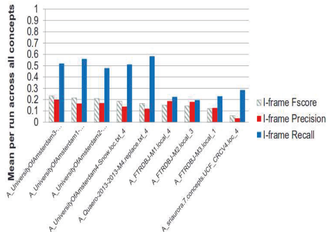
Fig. 11 2013: Temporal localization results by run
