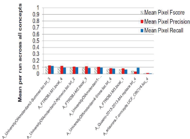
Fig. 17 2013: Spatial localization results by run
