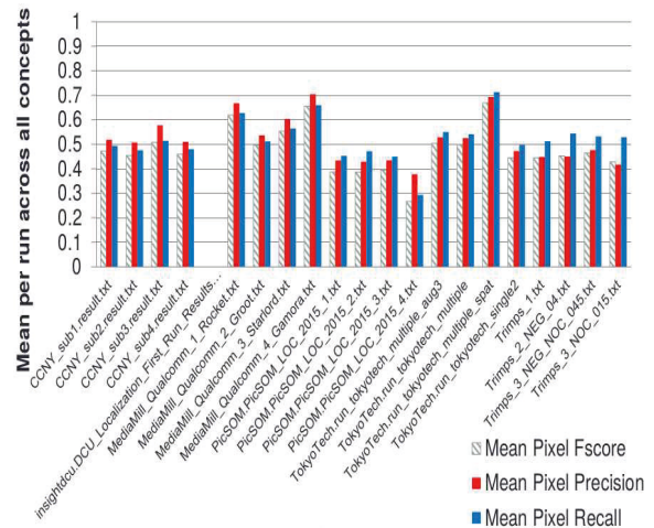
Fig. 18 2015: Spatial localization results by run
