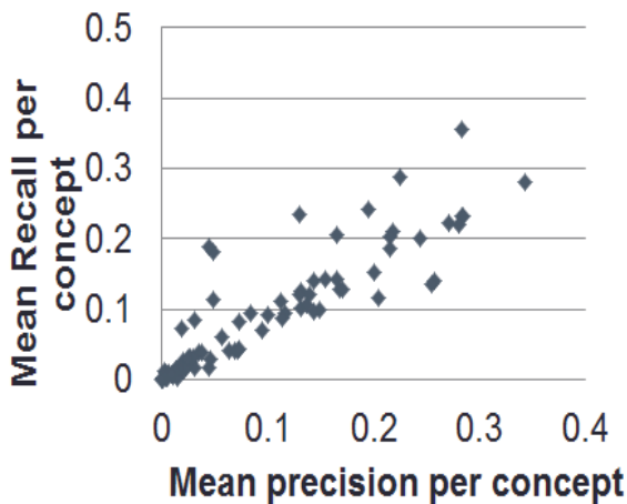
Fig. 19 2013: spatial precision and recall per concept for all teams
