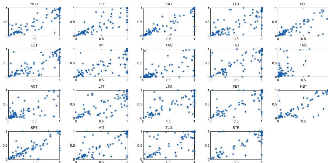
Fig. 15: The F -score of the run with a properly initial bounding box on the x -axes, and of the 20%-shifted initial bounding box on the y -axes.
