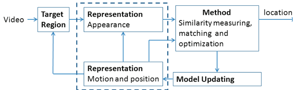
Fig. 1: Reference model of trackers with the five most important components.
