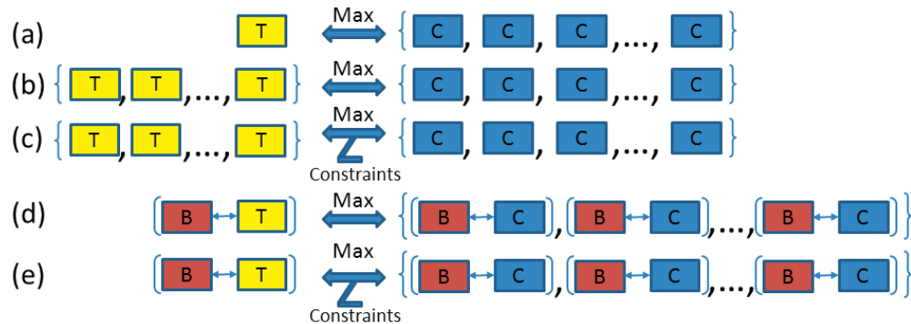
Fig. 5: Tracking methods employed in the trackers: (a) Matching; (b) Matching with extended appearance; (c) Matching with Constraints; (d) Discriminative classification and (e) Discriminative classification with constraints. T-boxes represent target instances. B-boxes represent local background instances. And C-boxes represent candidate targets.
