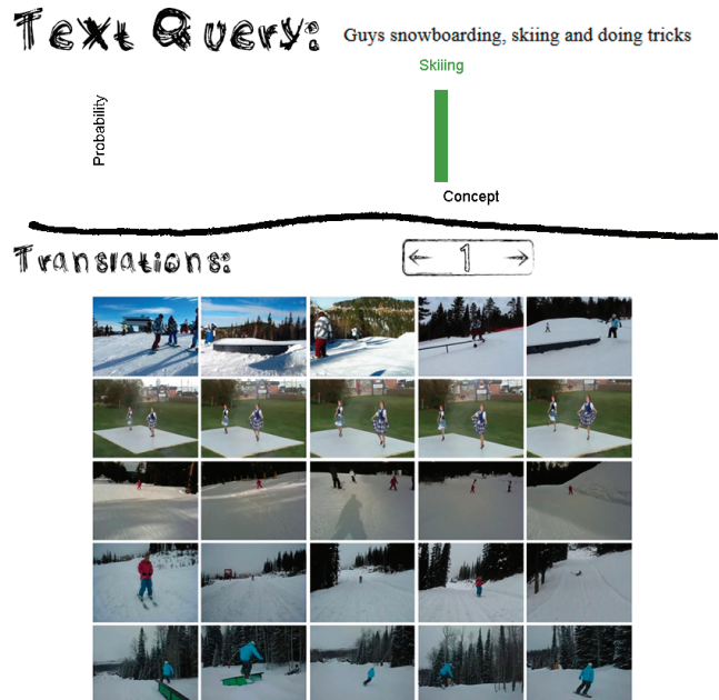
Figure 1: Sentence2Video : We automatically project an input sentence into a cross-media concept vocabulary, which is also used for representing video. The joint vocabulary allows us to translate a sentence to a video, and vice versa.
