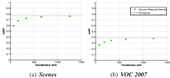
Figure 3. Experiment 3: Convex reduction parameters. Mean average precision given \lambda .
