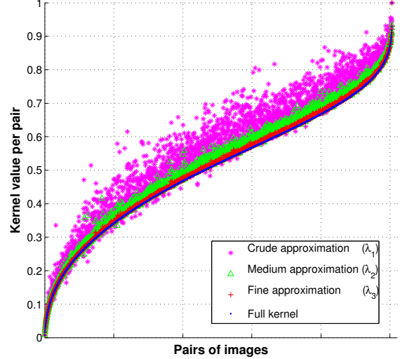
Figure 2. Kernel value distribution for various image pairs (best viewed in color). In blue we have the original kernel distance calculated. With the magenta, green and red we visualize convex reduced versions, that is \lambda_1 > \lambda_2 > \lambda_3 . The \lambda_1 approximations uses very few ( i.e. 66) dimensions, therefore accuracy of the kernel reconstruction is hurt.
