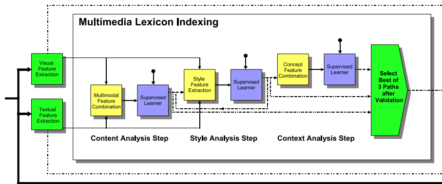
Fig. 2. Multimedia lexicon indexing is based on the semantic pathfinder [7]. In the detail from Fig. 1 we highlight its successive analysis steps. The semantic pathfinder selects for each concept a best path after validation.
