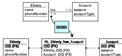
Figure 6 - Mapping one-to-many and many-to-many relationships
