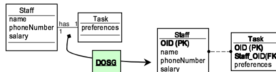
Figure 5. Mapping one-to-one class relationships
