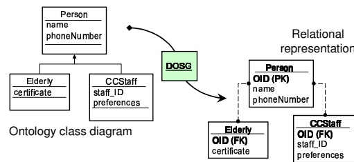
Figure 4 - Mapping the class hierarchies
